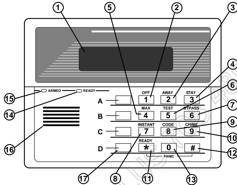
6139 2-LINE ALPHA KEYPAD
